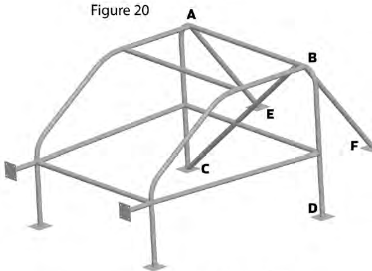
Figure 20 Diagonal brace may run B-C, A-D, A-F or B-E
