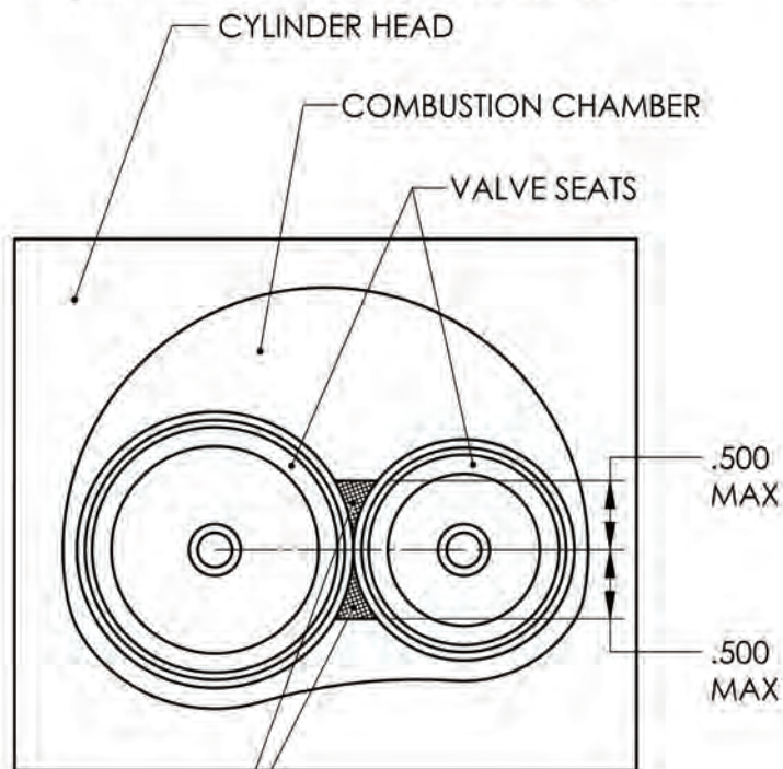
Figure 2 Aluminum Cylinder Head Repair Zone
